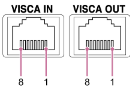
VISCA RS-422 pin layout (left: VISCA IN, right: VISCA OUT)
